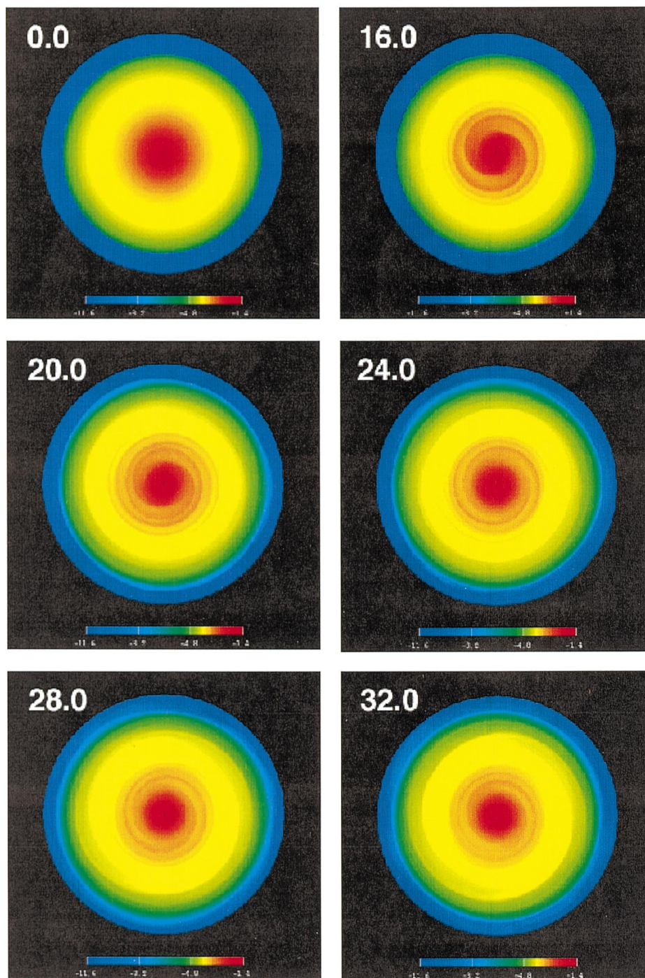
FIG. 10.—Time sequence of equatorial plane density images for the ADI + AV simulation. See Fig. 6.
